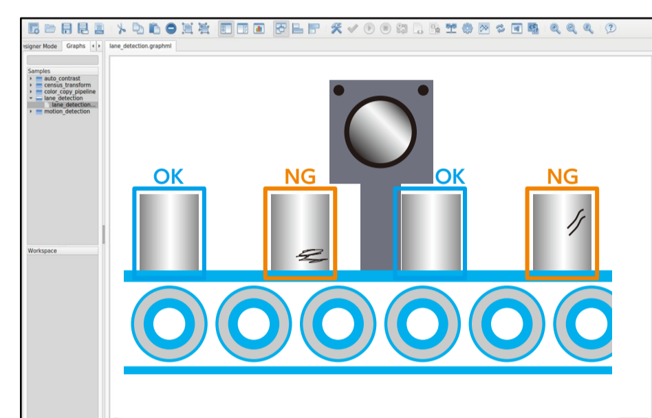
TED SDK
